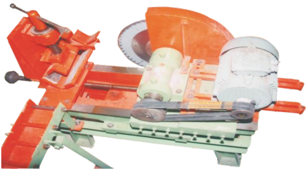
Billet Cutting Machine Dia. Cap. 75 mm x 175 mm
