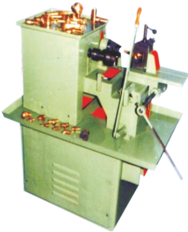
Double Head Turning & Threading Machine
